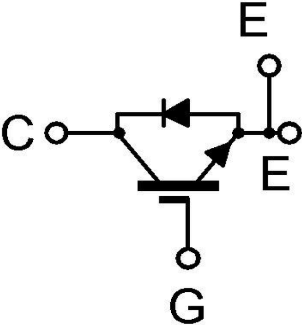
EQUIVALENT CIRCUIT
