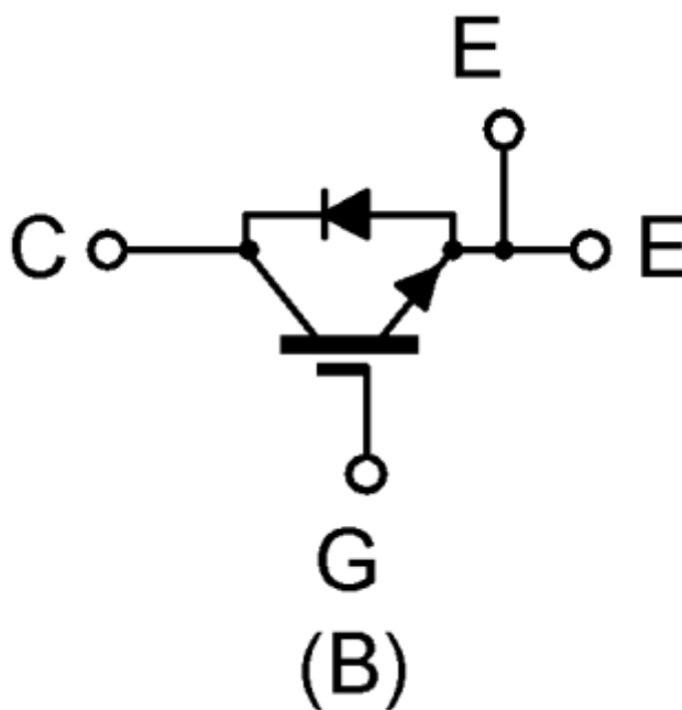
EQUIVALENT CIRCUIT
