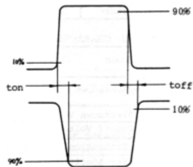
RESPONSE WAVEFORM
